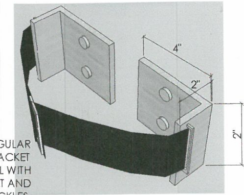
CO2 CYLINDER MOUNT DETAIL 2 A-1
