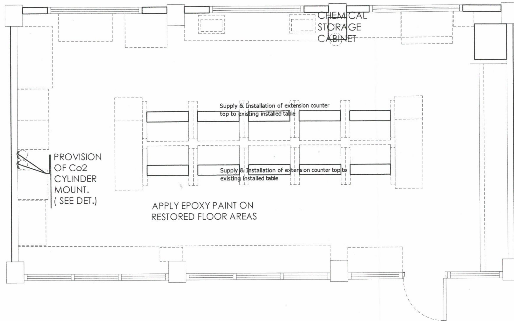
1 A-1 PROPOSED FLOOR PLAN SCALE: 1:50 MTS.
