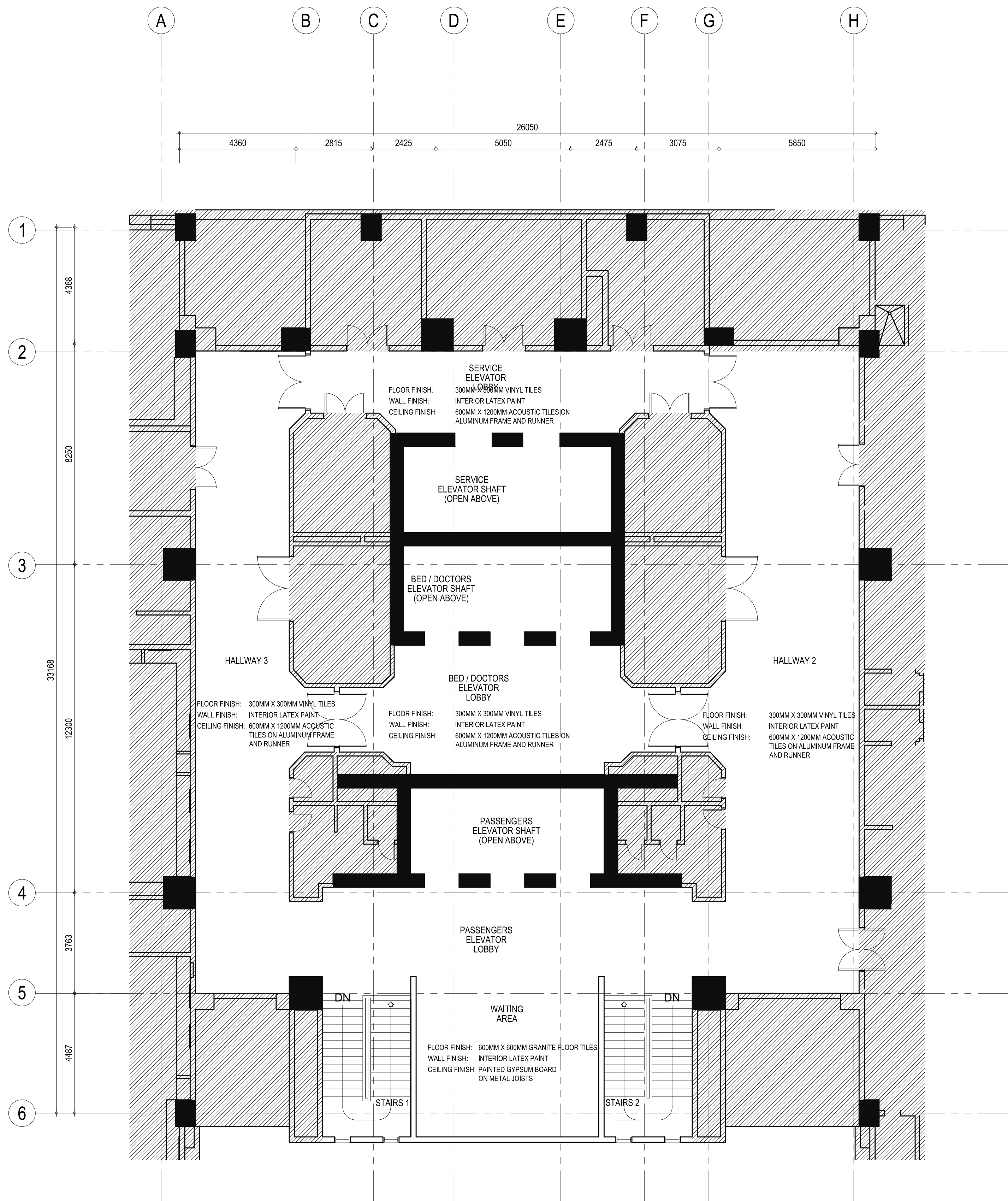
P05-ELEVATOR LOBBY 1 SEVENTH FLOOR - ASBUILT PLAN P05-A-107 SCALE: 1:100 MTS.
